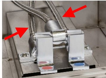
Tighten short flexible hoses in to foot pedal
